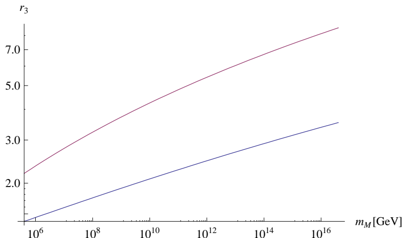
Figure 2. The RGE-factor r_3 as a function of the messenger scale for N_M = 1 (lower curve) and N_M = 3 (upper curve).
