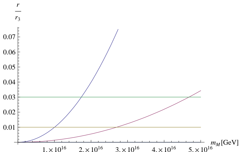
Figure 3. r/r_3 as a function of the messenger scale for N_M = 1 (upper curve) and N_M = 3 (lower curve) from eq. (6.3). The horizontal lines correspond to the FCNC upper bounds of eq. (4.1).
