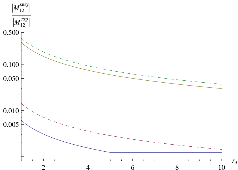
Figure 1. Maximum reach in B_d (solid) and B_s (dashed) mixing, |M_{12}^{\text{susy}}/M_{12}^{\text{exp}}| , as a function of the RGE-factor r_3 . The uppermost two curves correspond to \tan \beta = 30 and M_{A^0} = 200 GeV.
